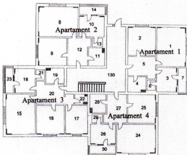
Parter
